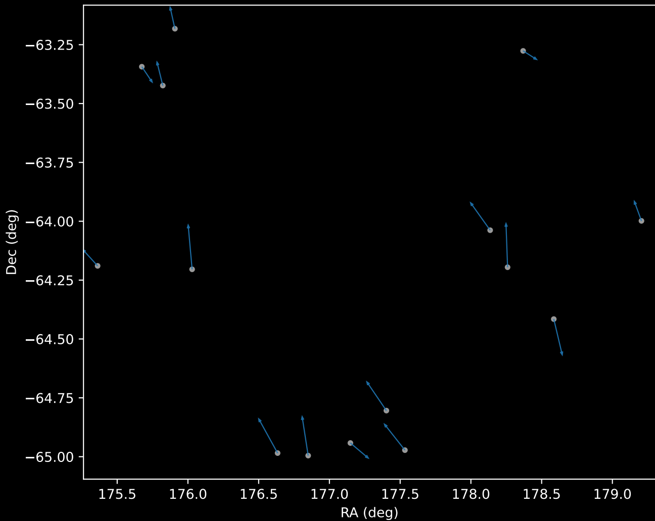
GALAH DR4 Cluster 0 Proper Motion Vectors (n=15)
