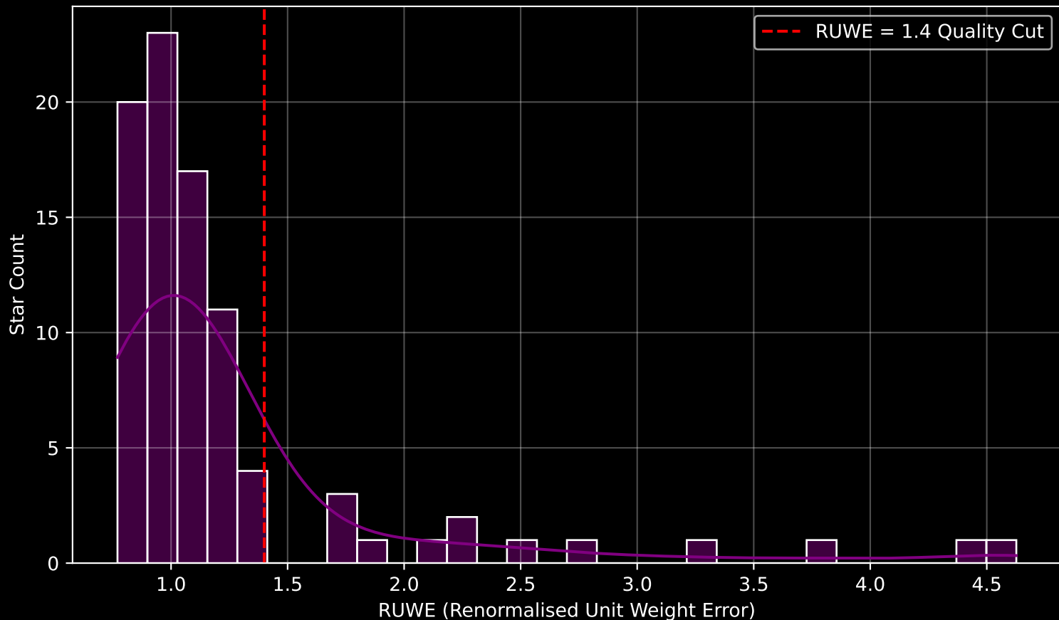
GALAH DR4 Field [7137] RUWE Distribution (n= 88)
