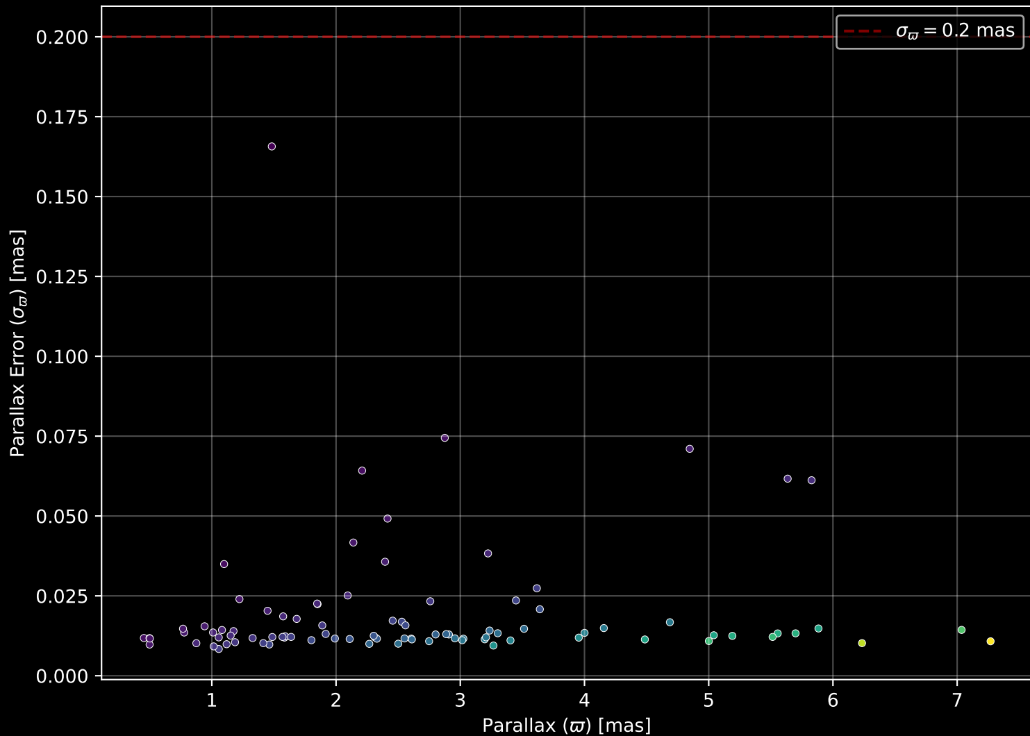
GALAH DR4 Field: [7137] Parallax Quality (n= 92)
