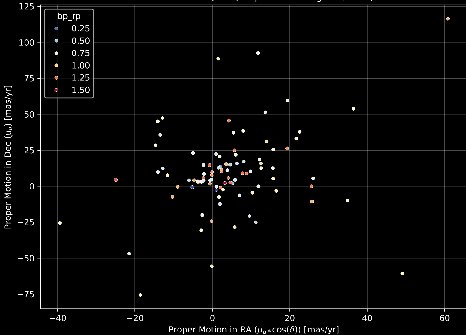
GALAH DR4 Field: [7137] Proper Motion Diagram (n= 92)
